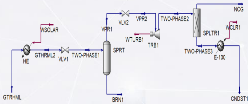
Geothermal-Solar Hybrid System (Zagy)
