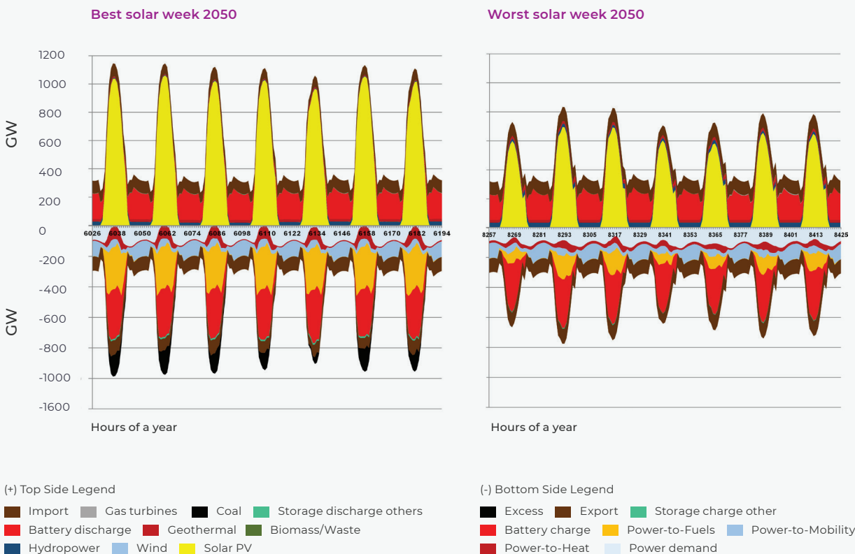
Figure 11: Hourly generation in best and worst solar weeks
