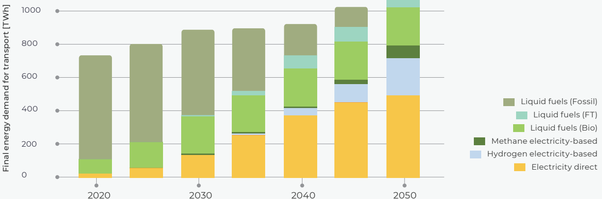
Figure 16: Final energy demand of the transport sector
