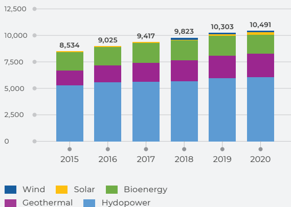
Figure 2: Renewable energy capacity and generation 2015-2020
