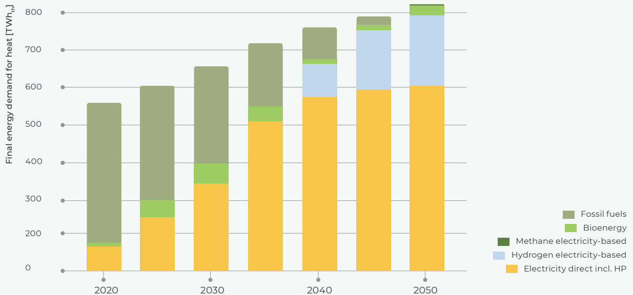
Figure 17: Final energy demand of the industry sector (heat)
