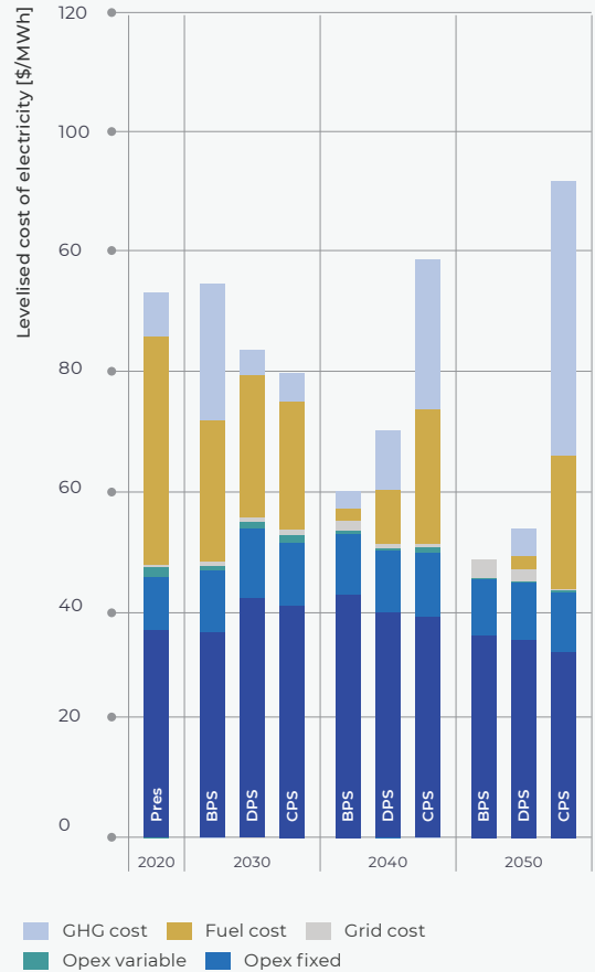
Figure 19: Levelized cost of electricity (LCOE)
